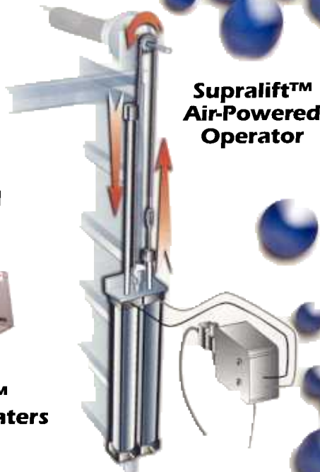
Vertical or Horizontal Mount
